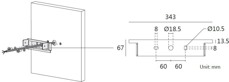
Secure the wall bracket
